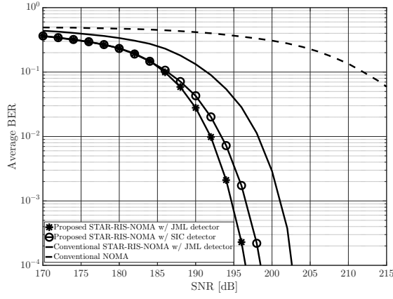
Fig. 2. BER performance of the LEO satellite communication system with STAR-RIS-NOMA when the number of Elements is 500, (d_{SL}, d_{TS}, d_{RS}) = (550\text{km}, 10\text{m}, 30\text{m}) .
